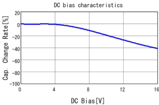
■ GRM033R71C182KA88 C-DC bias capchange, 25.0degC, AC1.
