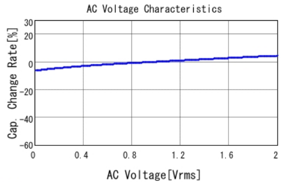
■ GRM033R71C182KA88 C-AC Voltage capchange, DCOV, 25.0d
