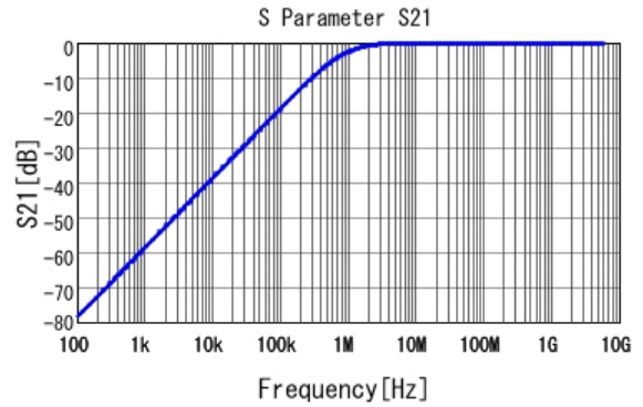
■ GRM033R71C182KA88 S21 DC0V, 25degC
