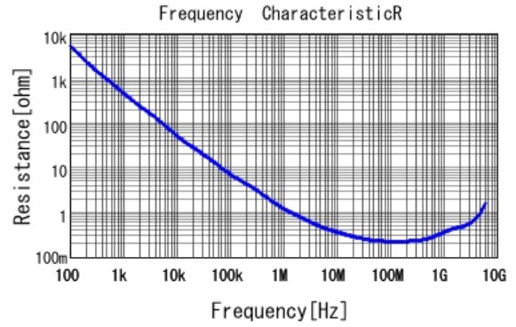
■ GRM033R71C182KA88 R DCOV, 25degC
