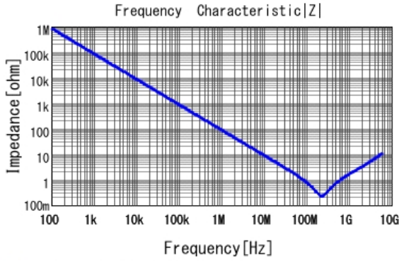
■ GRM033R71C182KA88 |Z| DCOV, 25degC
