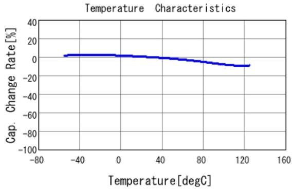
■ GRM033R71C222KA88 C-Temp. capchange, DC0.0V, AC1.0V rm
