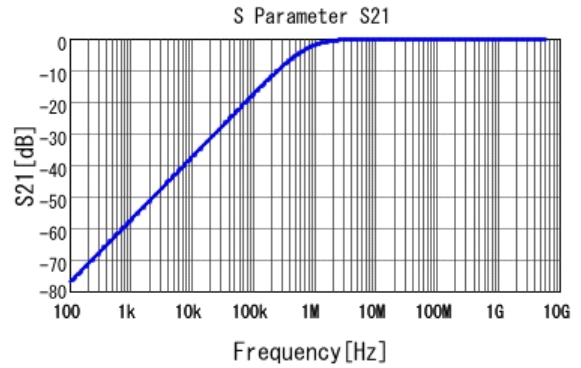
■ GRM033R71C222KA88 S21 DC0V, 25degC
