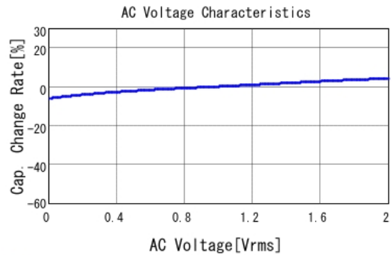
■ GRM033R71C332KA88 C-AC Voltage capchange, DCOV, 25.0d
