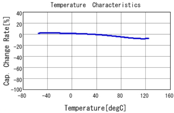
■ GRM033R71C332KA88 C-Temp. capchange, DC0.0V, AC1.0V rm
