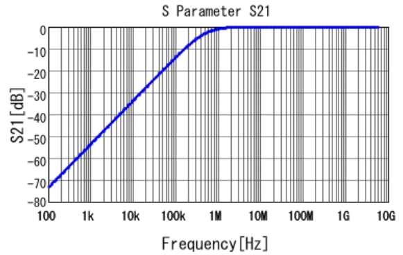
■ GRM033R71C332KA88 S21 DC0V, 25degC
