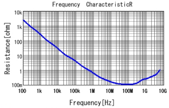
■ GRM033R71C332KA88 R DCOV, 25degC
