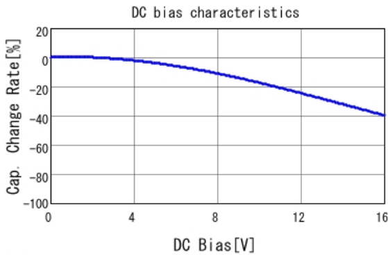
■ GRM033R71C332KA88 C-DC bias capchange, 25.0degC, AC1.
