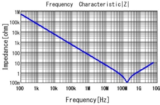
■ GRM033R71C332KA88 |Z| DCOV, 25degC
