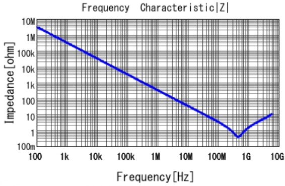
■ GRM033R71C471KA01 |Z| DCOV, 25degC
