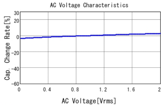
■ GRM033R71C471KA01 C-AC Voltage capchange, DCOV, 25.0d
