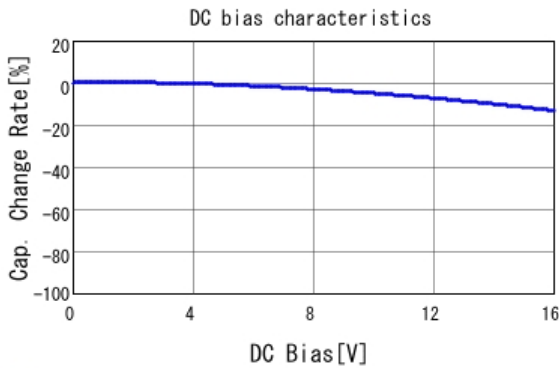
■ GRM033R71C471KA01 C-DC bias capchange, 25.0degC, AC1.
