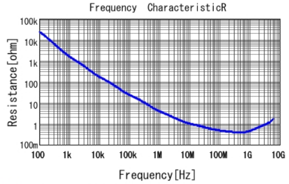
■ GRM033R71C471KA01 R DCOV, 25degC
