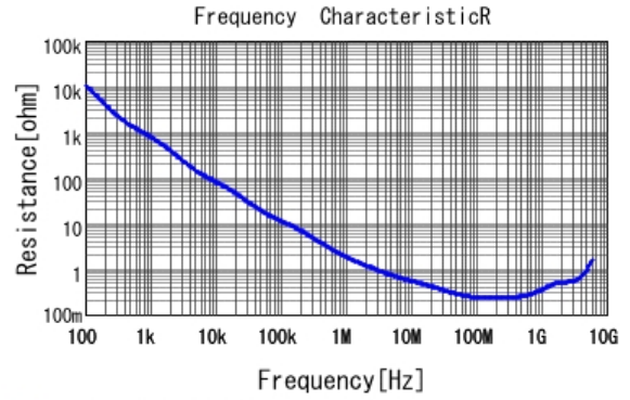
■ GRM033R71E102KA01 R DCOV, 25degC
