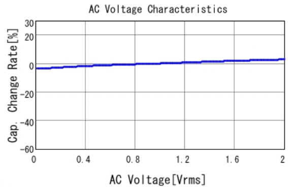
■ GRM033R71E102KA01 C-AC Voltage capchange, DCOV, 25.0d
