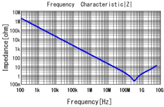
■ GRM033R71E102KA01 |Z| DCOV, 25degC
