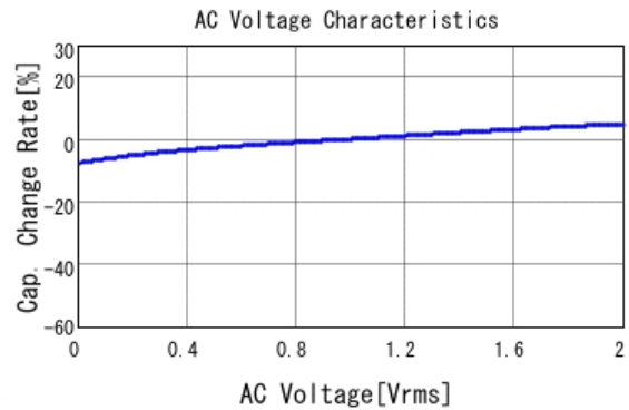
■ GRM033R71E103KE14 C-AC Voltage capchange, DCOV, 25.0d
