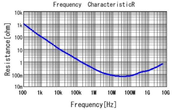
■ GRM033R71E103KE14 R DCOV, 25degC
