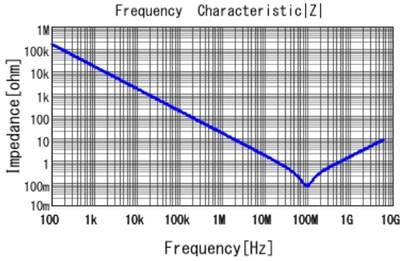
■ GRM033R71E103KE14 |Z| DCOV, 25degC
