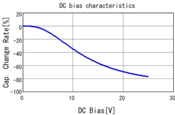
■ GRM033R71E103KE14 C-DC bias capchange, 25.0degC, AC1.
