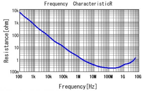
■ GRM033R71E152KA01 R DCOV, 25degC
