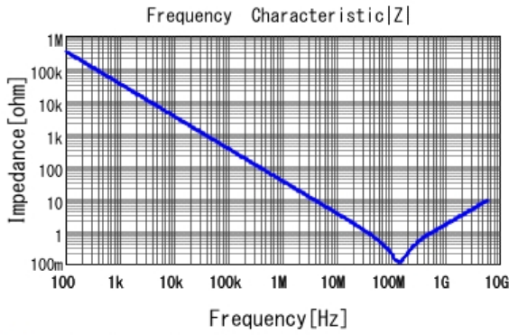
■ GRM033R71E472KE14 |Z| DCOV, 25degC
