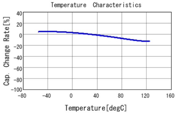
■ GRM033R71E472KE14 C-Temp. capchange, DC0.0V, AC1.0Vrm
