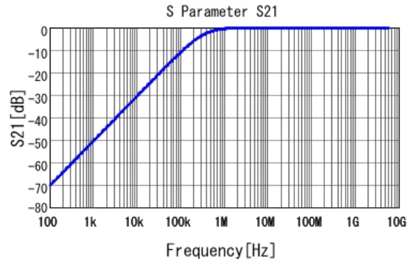
■ GRM033R71E472KE14 S21 DC0V, 25degC
