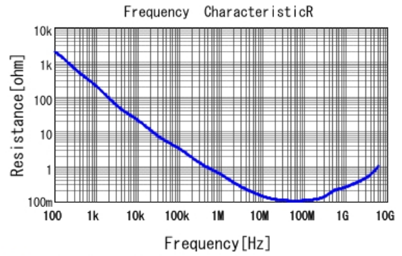
■ GRM033R71E472KE14 R DCOV, 25degC
