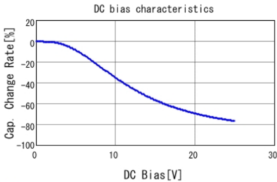
■ GRM033R71E472KE14 C-DC bias capchange, 25.0degC, AC1.
