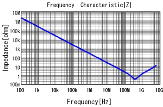
■ GRM033R71E821KA01 |Z| DCOV, 25degC
