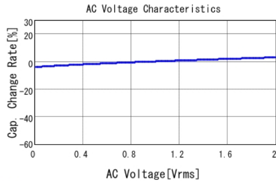
■ GRM033R71E821KA01 C-AC Voltage capchange, DCOV, 25.0d
