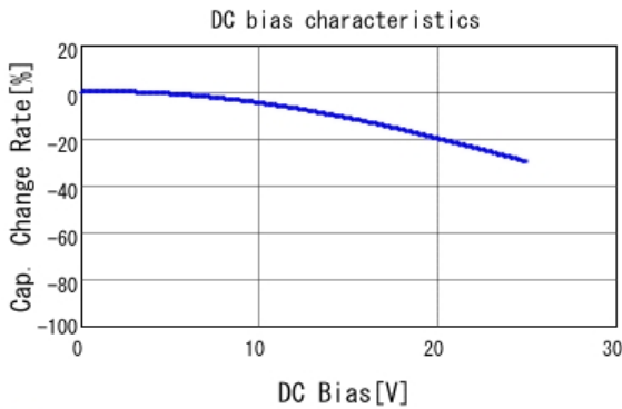
■ GRM033R71E821KA01 C-DC bias capchange, 25.0degC, AC1.
