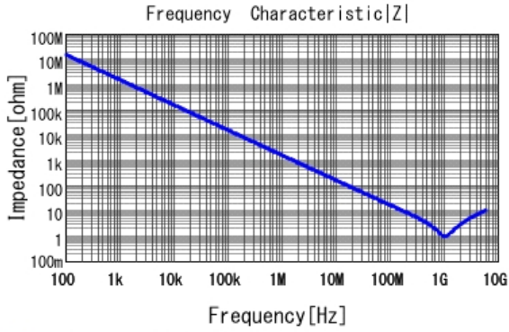
■ GRM033R71H101KA12 |Z| DCOV, 25degC
