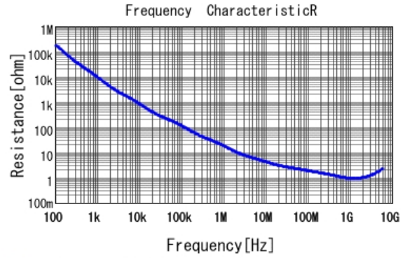
■ GRM033R71H101KA12 R DCOV, 25degC
