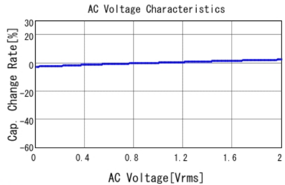
■ GRM033R71H101KA12 C-AC Voltage capchange, DCOV, 25.0d
