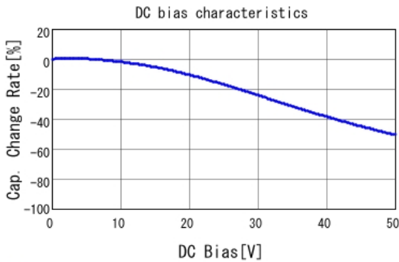
■ GRM033R71H101KA12 C-DC bias capchange, 25.0degC, AC1.
