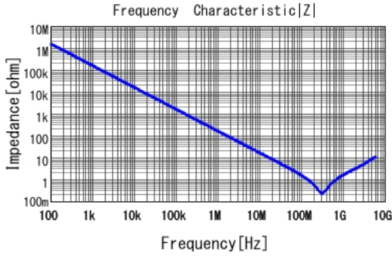
■ GRM033R71H102KA12 |Z| DCOV, 25degC
