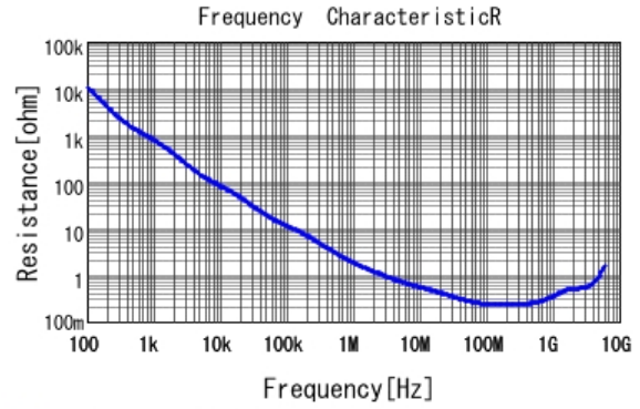
■ GRM033R71H102KA12 R DCOV, 25degC
