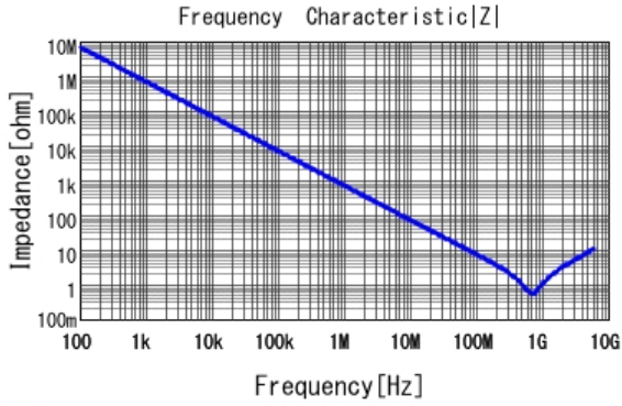
■ GRM033R71H221KA12 |Z| DCOV, 25degC
