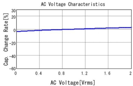
■ GRM033R71H471KA12 C-AC Voltage capchange, DCOV, 25.0d
