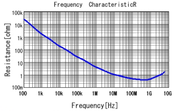
■ GRM033R71H471KA12 R DCOV, 25degC
