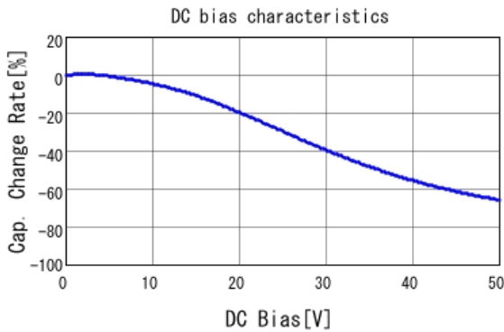
■ GRM033R71H471KA12 C-DC bias capchange, 25.0degC, AC1.
