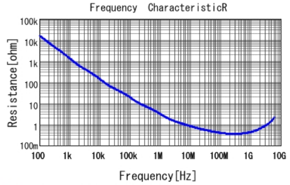
■ GRM033R71H681KA12 R DCOV, 25degC
