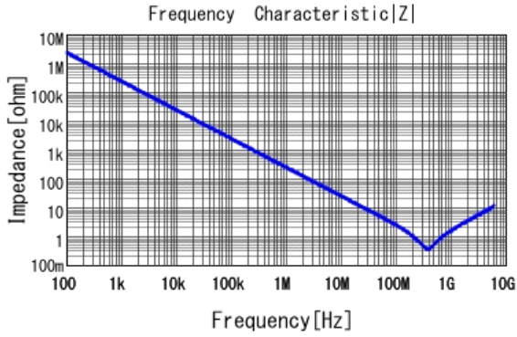
■ GRM033R71H681KA12 |Z| DCOV, 25degC
