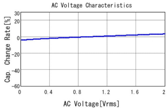
■ GRM033R71H681KA12 C-AC Voltage capchange, DCOV, 25.0d
