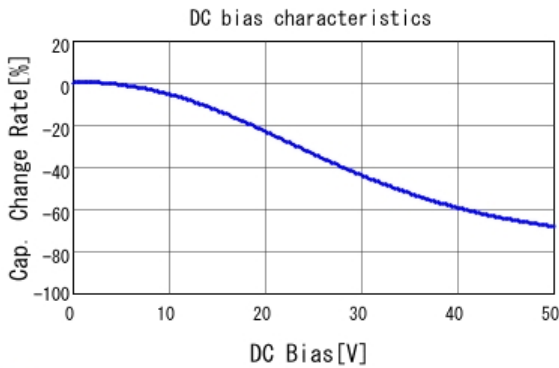
■ GRM033R71H681KA12 C-DC bias capchange, 25.0degC, AC1.
