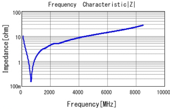
■ GRM1552C1H151JA01 |Z| DCOV, 20degC
