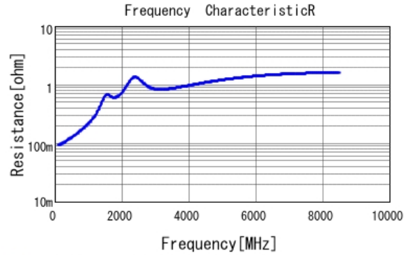
■ GRM1552C1H151JA01 R DCOV, 20degC
