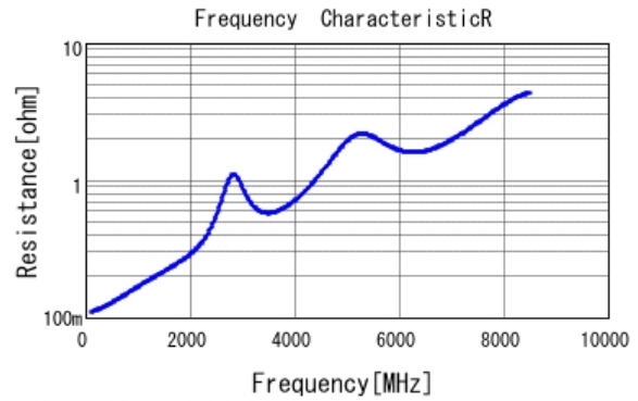
■ GRM1552C1H390JA01 R DCOV, 20degC
