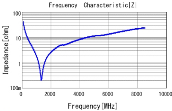
■ GRM1552C1H390JA01 |Z| DCOV, 20degC
