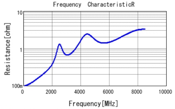
■ GRM1552C1H470JA01 R DCOV, 20degC
