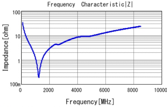
■ GRM1552C1H470JA01 |Z| DCOV, 20degC
