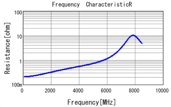
■ GRM1552C1H5R0BA01 R DCOV, 20degC
