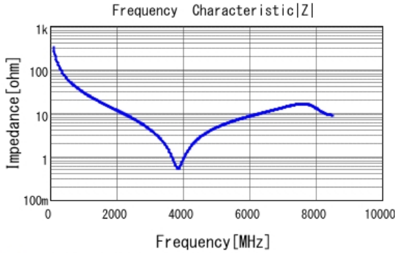
■ GRM1552C1H5R0BA01 |Z| DCOV, 20degC
