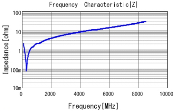
■ GRM1552C1H681JA01 |Z| DCOV, 20degC
