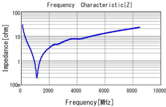
■ GRM1552C2A560JA01 |Z| DCOV, 20degC
