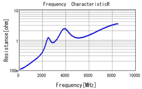
■ GRM1552C2A560JA01 R DCOV, 20degC
