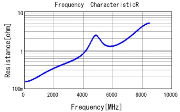
■ GRM1555C1E150JA01 R DCOV, 25degC
