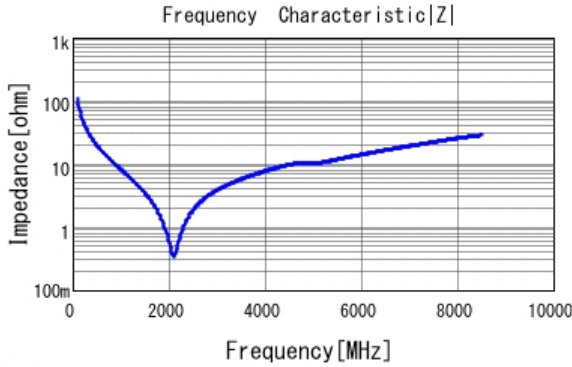
■ GRM1555C1E150JA01 |Z| DCOV, 25degC
