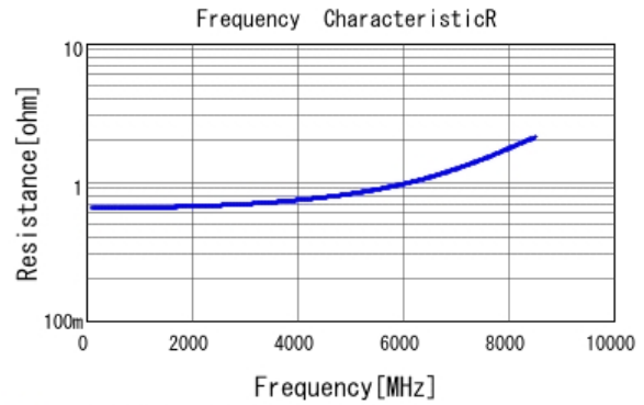
■ GRM1555C1E1R2CA01 R DCOV, 25degC
