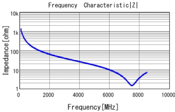
■ GRM1555C1E1R2CA01 |Z| DCOV, 25degC
