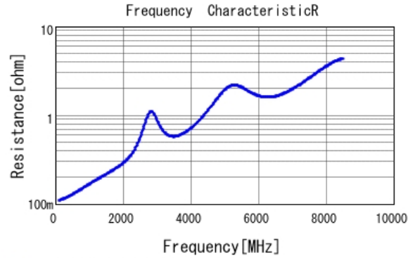
■ GRM1555C1E390JA01 R DCOV, 25degC
