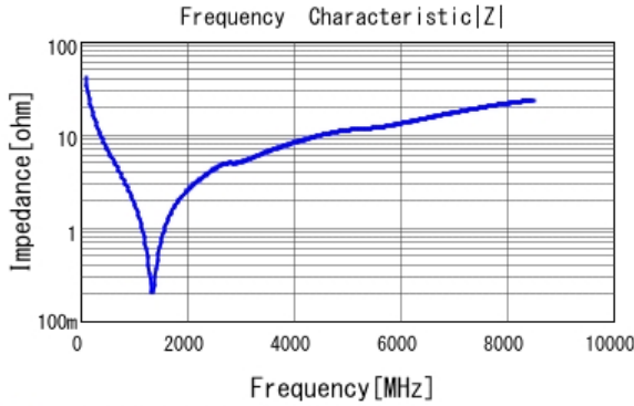
■ GRM1555C1E390JA01 |Z| DCOV, 25degC
