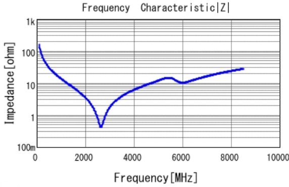
■ GRM1555C1H100JA01 |Z| DCOV, 25degC
