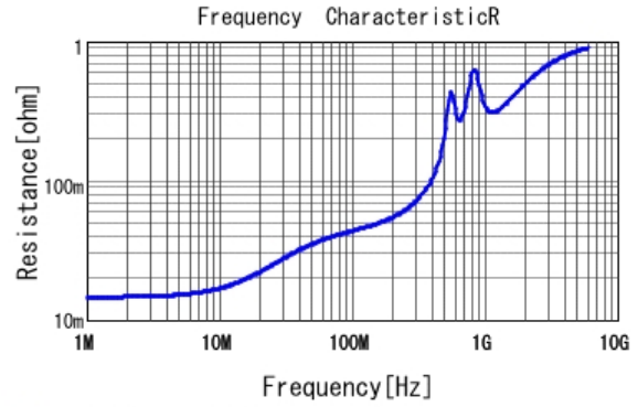
■ GRM1555C1H102JA01 R DCOV, 25degC
