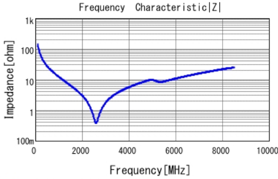
■ GRM1555C1H110JA01 |Z| DCOV, 25degC
