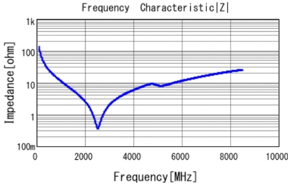
■ GRM1555C1H120JA01 |Z| DCOV, 25degC
