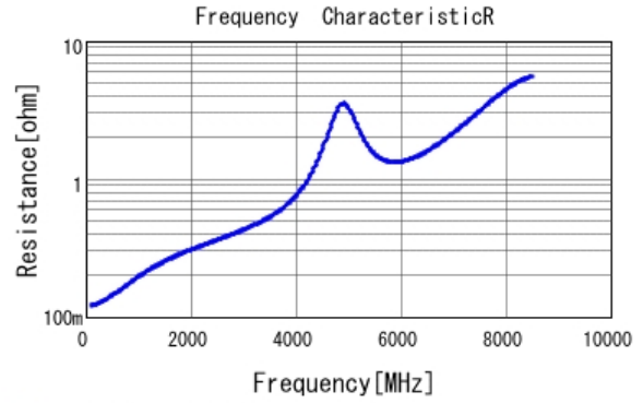
■ GRM1555C1H120JA01 R DCOV, 25degC
