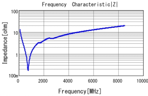
■ GRM1555C1H121GA01 |Z| DCOV, 25degC
