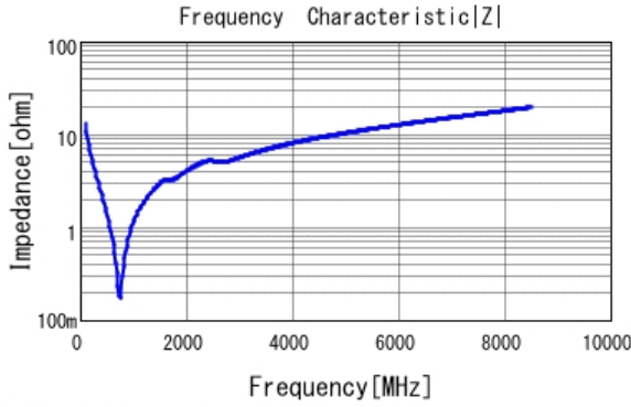
■ GRM1555C1H121JA01 |Z| DCOV, 25degC
