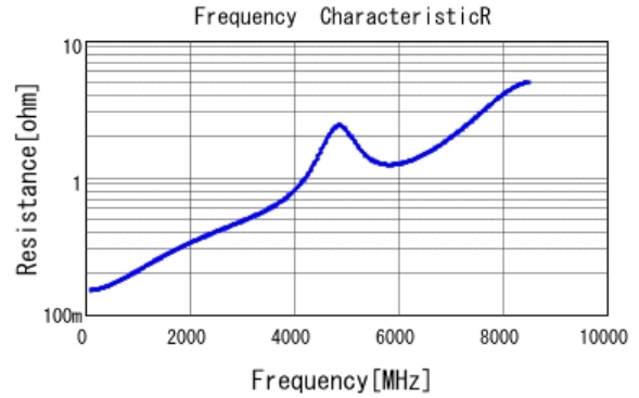
■ GRM1555C1H150JA01 R DCOV, 25degC
