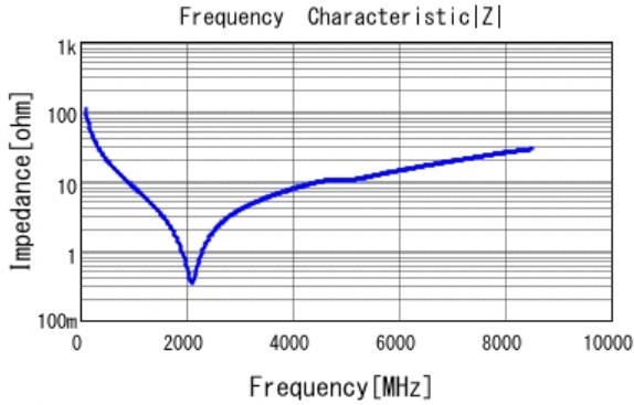
■ GRM1555C1H150JA01 |Z| DCOV, 25degC
