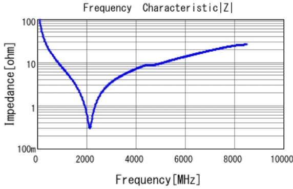
■ GRM1555C1H160JA01 |Z| DCOV, 25degC
