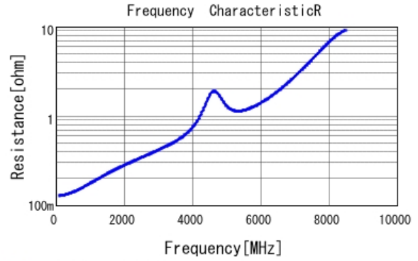
■ GRM1555C1H160JA01 R DCOV, 25degC
