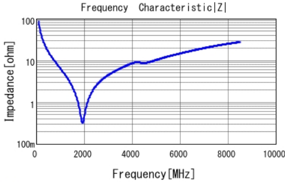
■ GRM1555C1H180GA01 |Z| DCOV, 25degC
