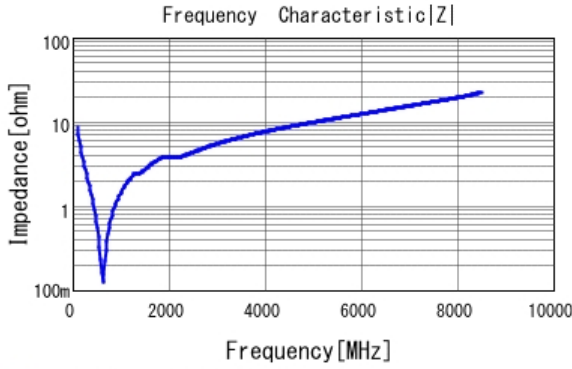
■ GRM1555C1H181GA01 |Z| DCOV, 25degC
