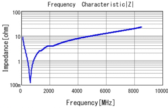
■ GRM1555C1H181JA01 |Z| DCOV, 25degC
