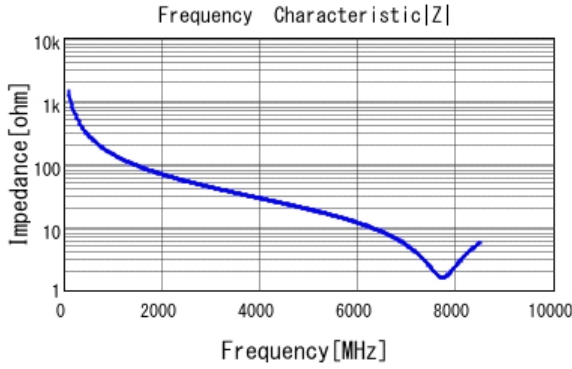
■ GRM1555C1H1R1BA01 |Z| DCOV, 25degC
