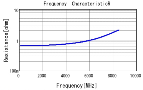
■ GRM1555C1H1R1BA01 R DCOV, 25degC
