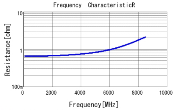
■ GRM1555C1H1R2CA01 R DCOV, 25degC
