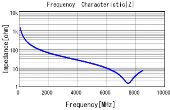
■ GRM1555C1H1R2WA01 |Z| DCOV, 25degC
