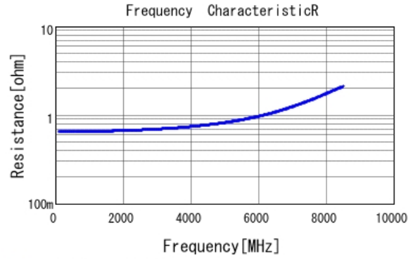
■ GRM1555C1H1R2WA01 R DCOV, 25degC
