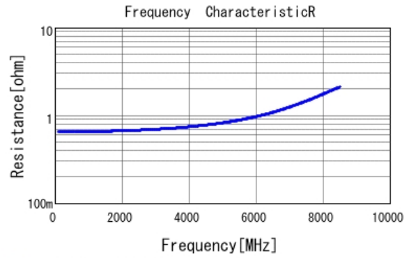
■ GRM1555C1H1R3WA01 R DCOV, 25degC
