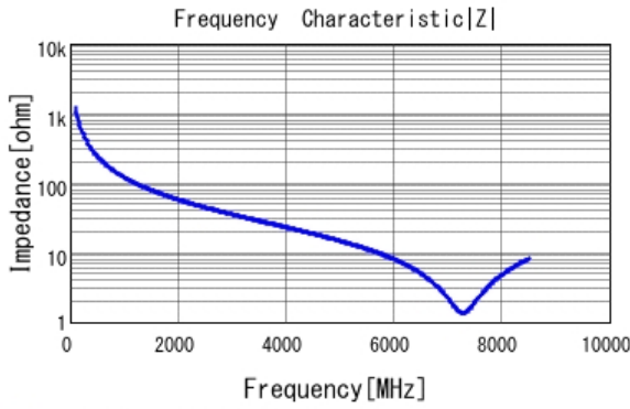
■ GRM1555C1H1R3WA01 |Z| DCOV, 25degC
