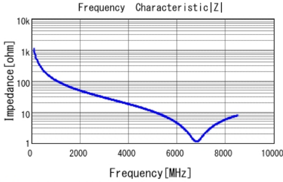
■ GRM1555C1H1R5BA01 |Z| DC0V, 25degC
