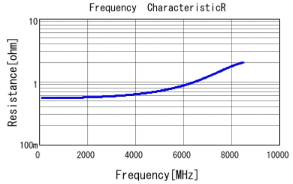
■ GRM1555C1H1R5BA01 R DC0V, 25degC
