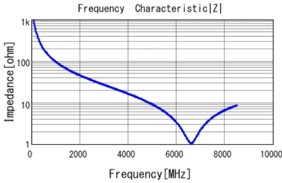
■ GRM1555C1H1R6BA01 |Z| DC0V, 25degC
