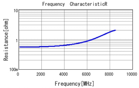
■ GRM1555C1H1R6BA01 R DC0V, 25degC
