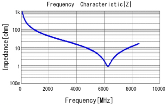
■ GRM1555C1H1R8BA01 |Z| DCOV, 25degC
