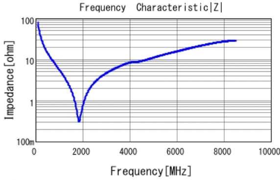
■ GRM1555C1H200JA01 |Z| DCOV, 25degC
