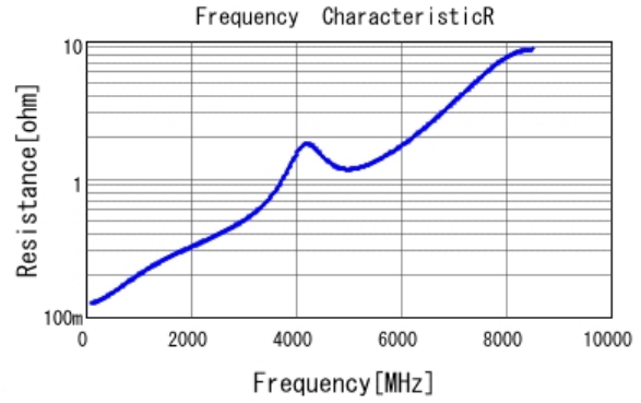
■ GRM1555C1H200JA01 R DCOV, 25degC
