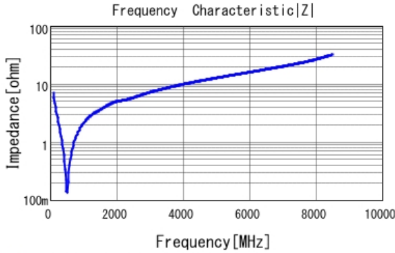
■ GRM1555C1H221JA01 |Z| DCOV, 25degC
