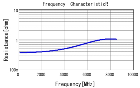
■ GRM1555C1H2R0CA01 R DCOV, 25degC
