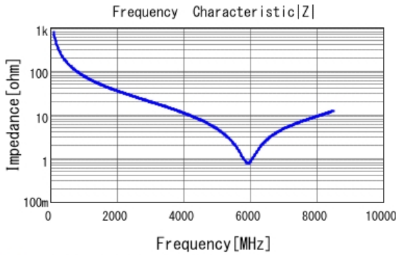
■ GRM1555C1H2R0CA01 |Z| DCOV, 25degC
