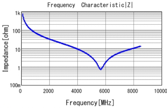
■ GRM1555C1H2R2CA01 |Z| DCOV, 25degC
