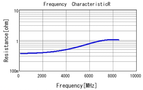
■ GRM1555C1H2R2CA01 R DCOV, 25degC
