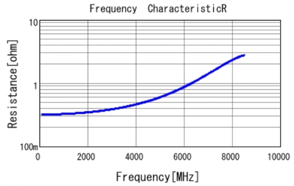
■ GRM1555C1H2R4CA01 R DCOV, 25degC
