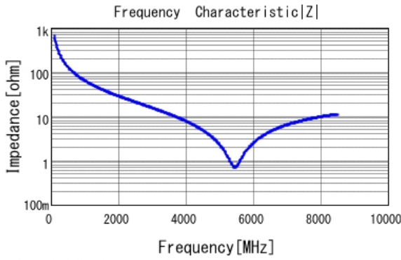
■ GRM1555C1H2R4CA01 |Z| DCOV, 25degC
