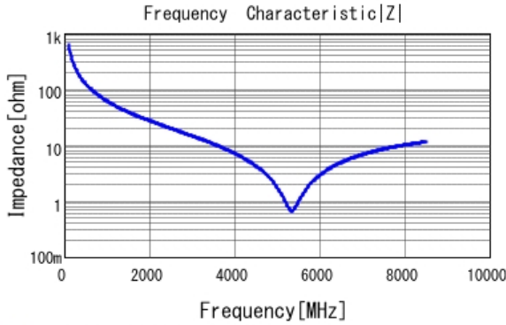
■ GRM1555C1H2R5BA01 |Z| DCOV, 25degC
