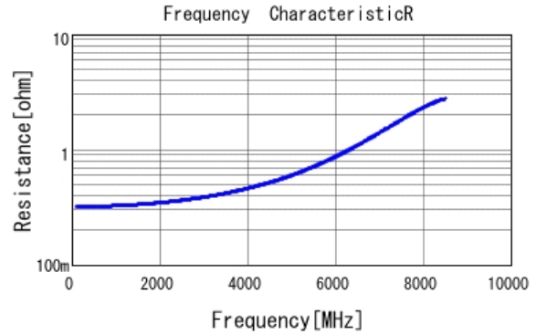
■ GRM1555C1H2R5BA01 R DCOV, 25degC
