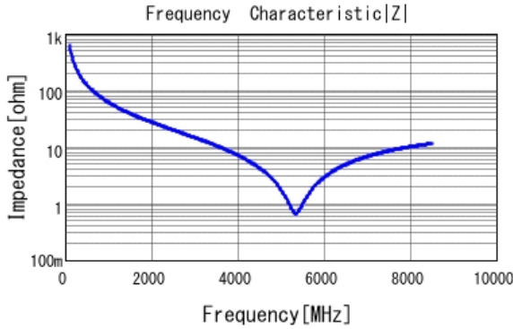
■ GRM1555C1H2R5CA01 |Z| DCOV, 25degC
