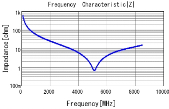
■ GRM1555C1H2R7BA01 |Z| DCOV, 25degC
