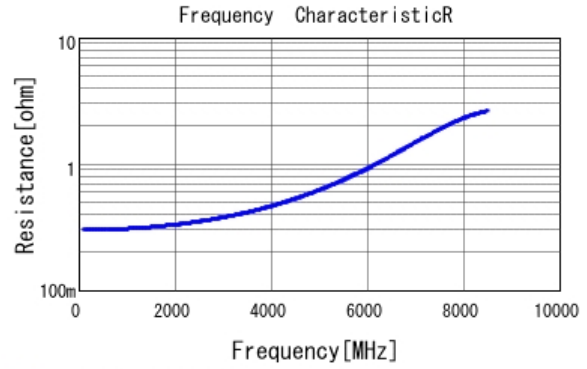
■ GRM1555C1H2R7BA01 R DCOV, 25degC
