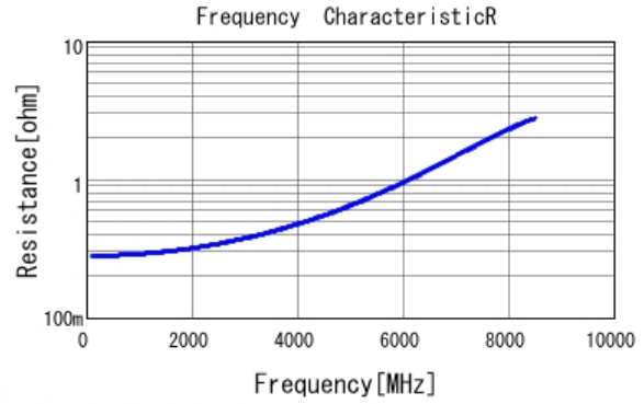
■ GRM1555C1H2R9BA01 R DCOV, 25degC
