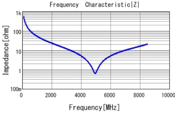
■ GRM1555C1H2R9BA01 |Z| DCOV, 25degC
